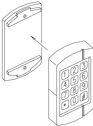
PIN Keypad mounting "firm click" connection
